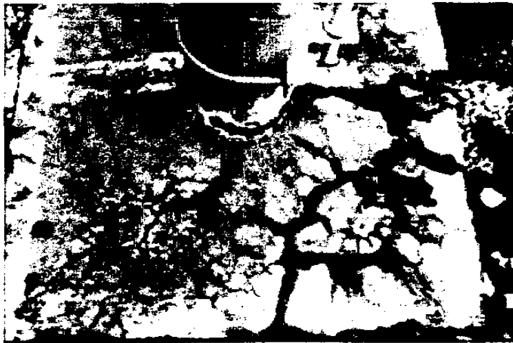
Fig. 4—Cracking in cast-in-situ concrete pedestal for electric power line.
